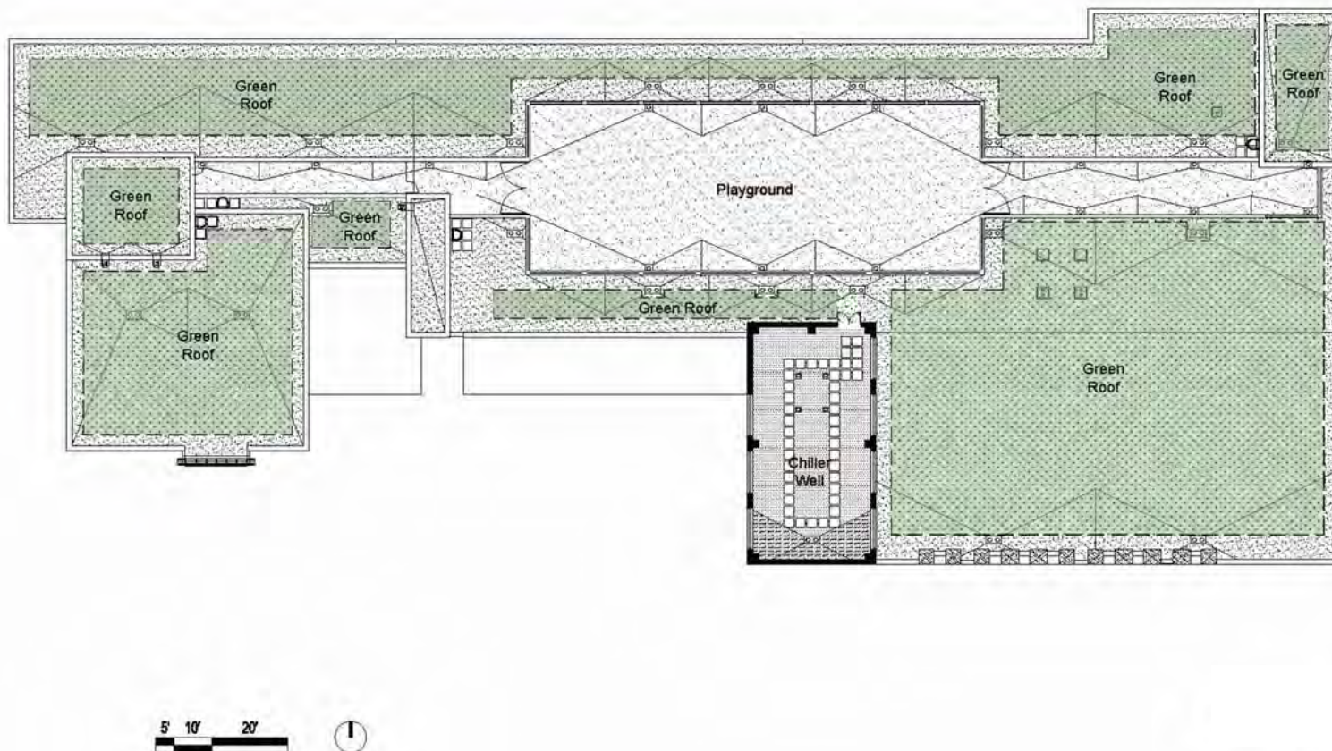
GREEN ROOF PLAN
