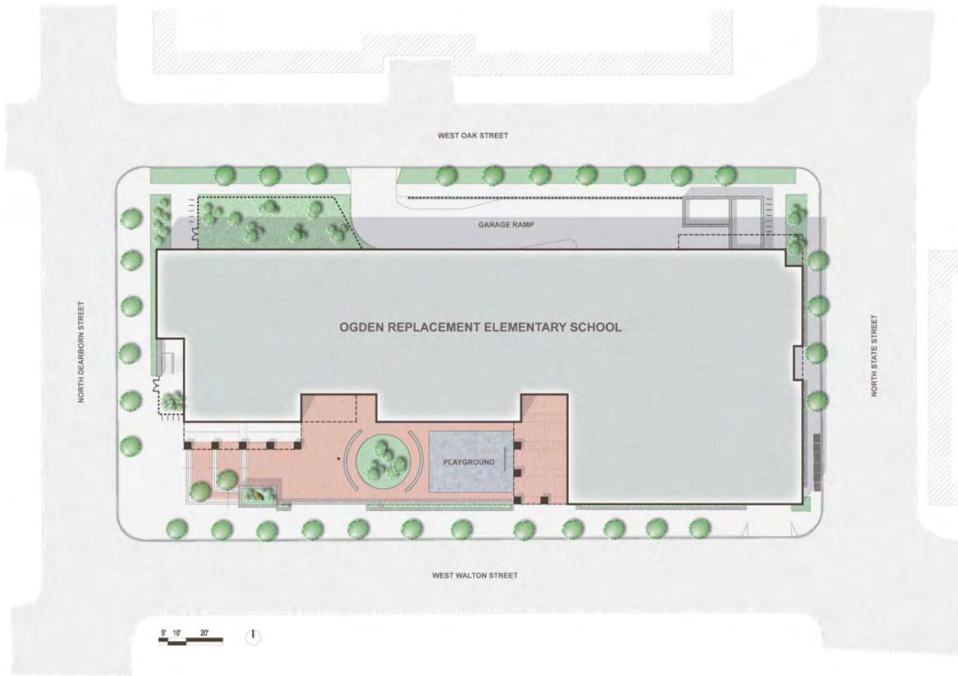
SITE PLAN
