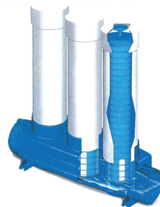
Bio-Dynamic dry chlorine feeder and tablets
