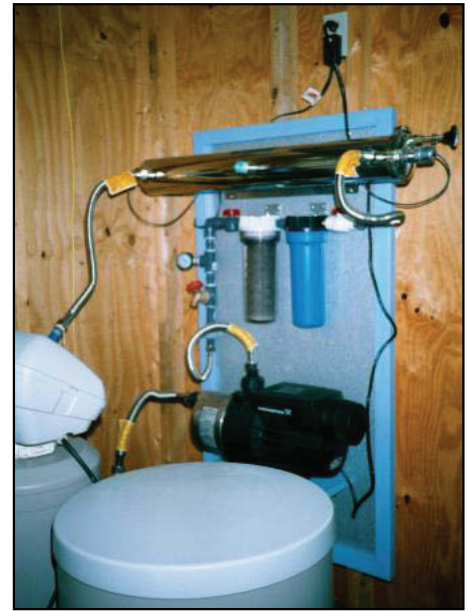
UV Light (top horizontal cylinder) Texas Rainwater Manual
