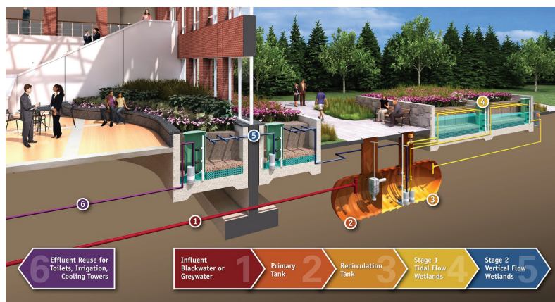
Living Machine® Sample Diagram. www.livingmachines.com/about/howitworks
