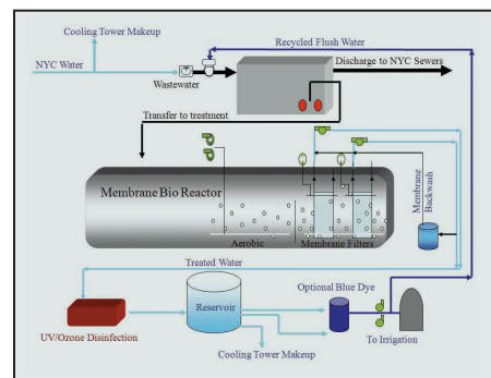
The Solaire's blackwater system
