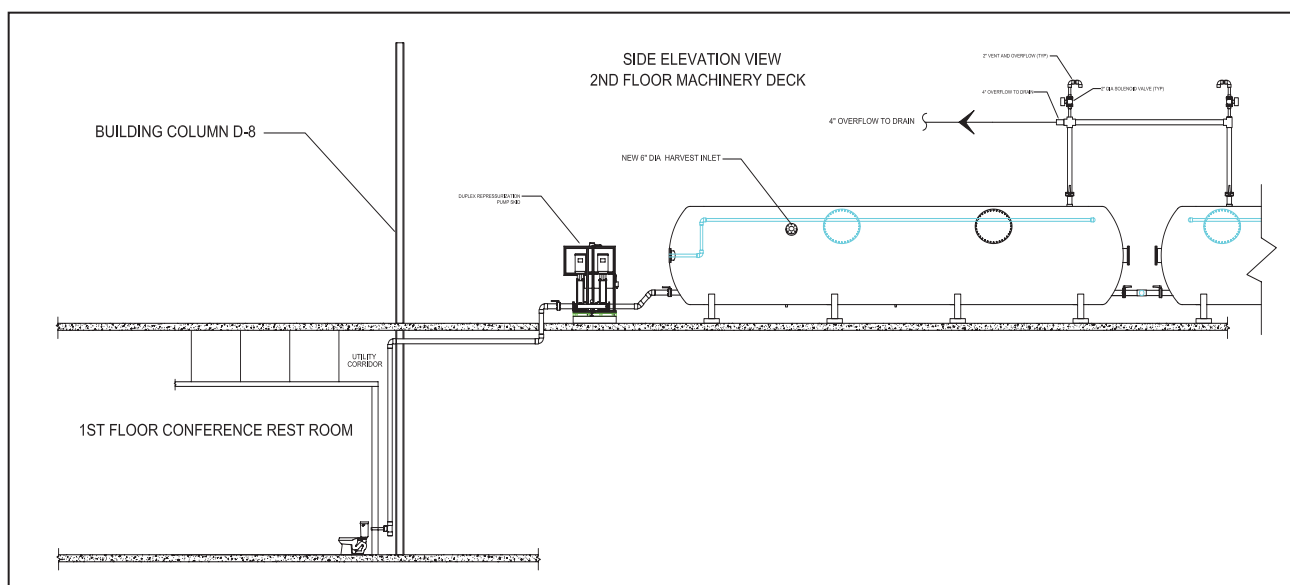
Plumbing Schematic
